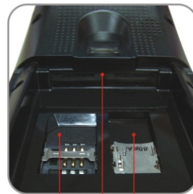
SIM card SAM slots microSD
