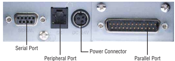
PP6800C 3-in-1 [Parallel]
