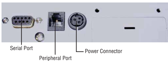
PP6800S 2-in-1 [Serial]
