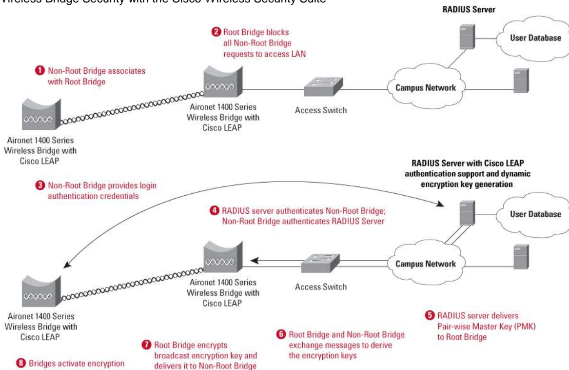
Figure 3. Wireless Bridge Security with the Cisco Wireless Security Suite
