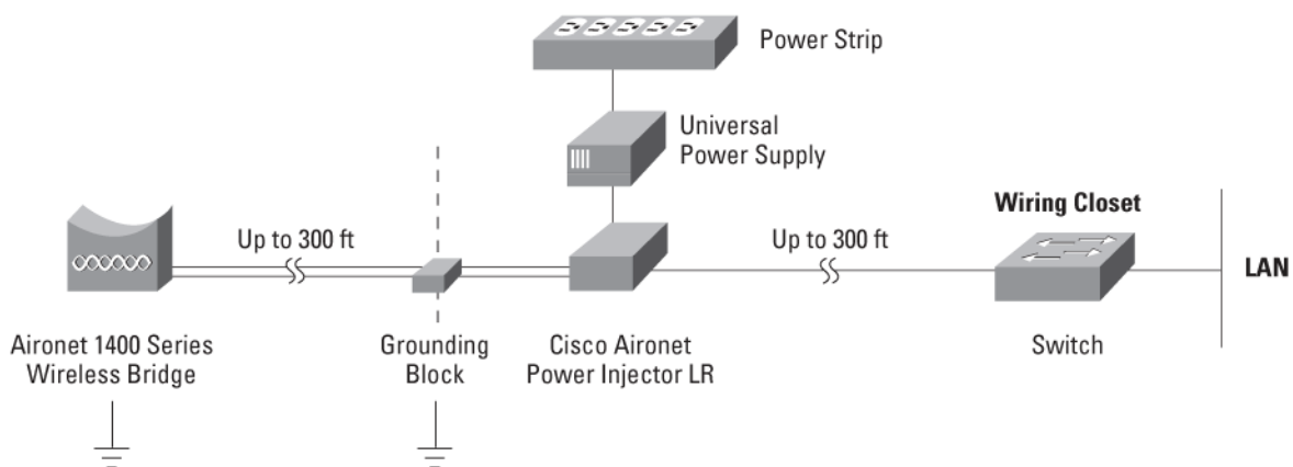
Figure 6. Power Injector Distance Extension
