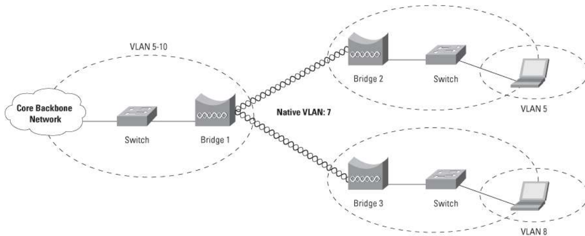
Figure 4. VLAN Configuration for Wireless Bridges
