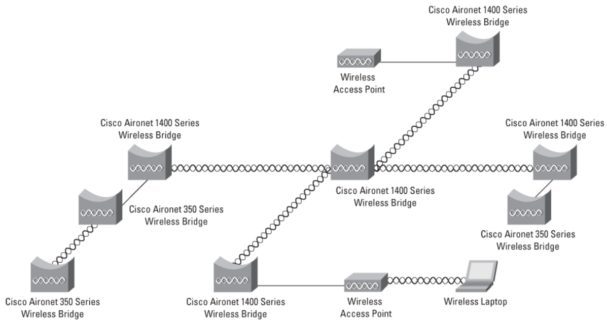
Figure 2. Public Safety Network Utilizing Wireless Bridges
