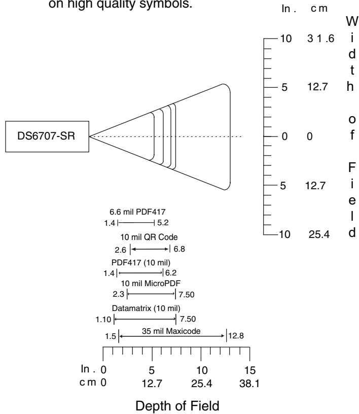
Figure 2-8 Symbol DS6707 Standard Range Decode Zone for 2D Bar Codes
