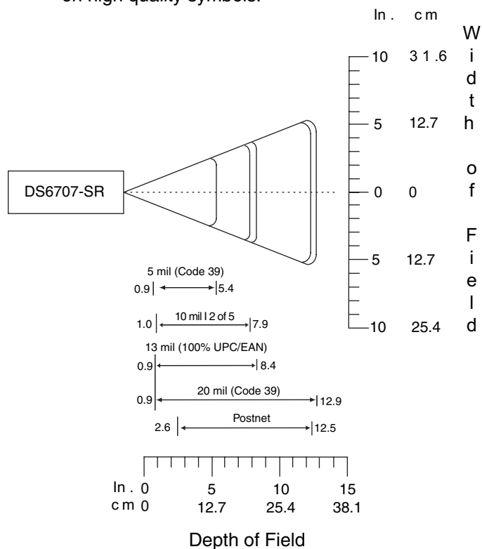
Figure 2-7 Symbol DS6707 Standard Range Decode Zone for 1D Bar Codes
