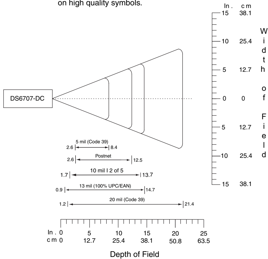
Figure 2-9 Symbol DS6707 Digital Imager Scanner Document Capture Decode Zone for 1D Bar Codes
