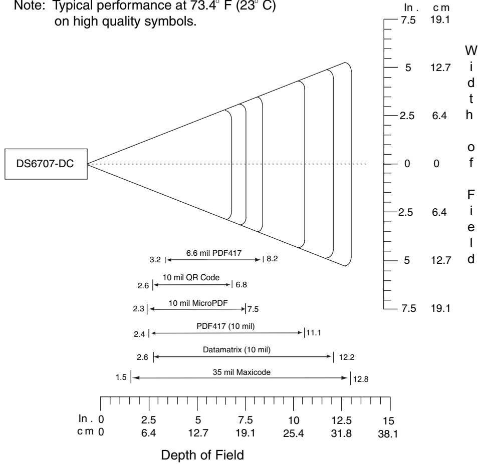
Figure 2-10 Symbol DS6707 Digital Imager Scanner Document Capture Decode Zone for 2D Bar Codes
